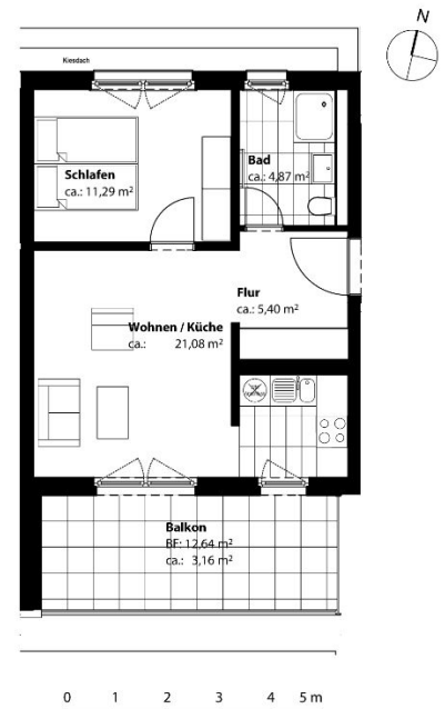
Grundriss_SW
